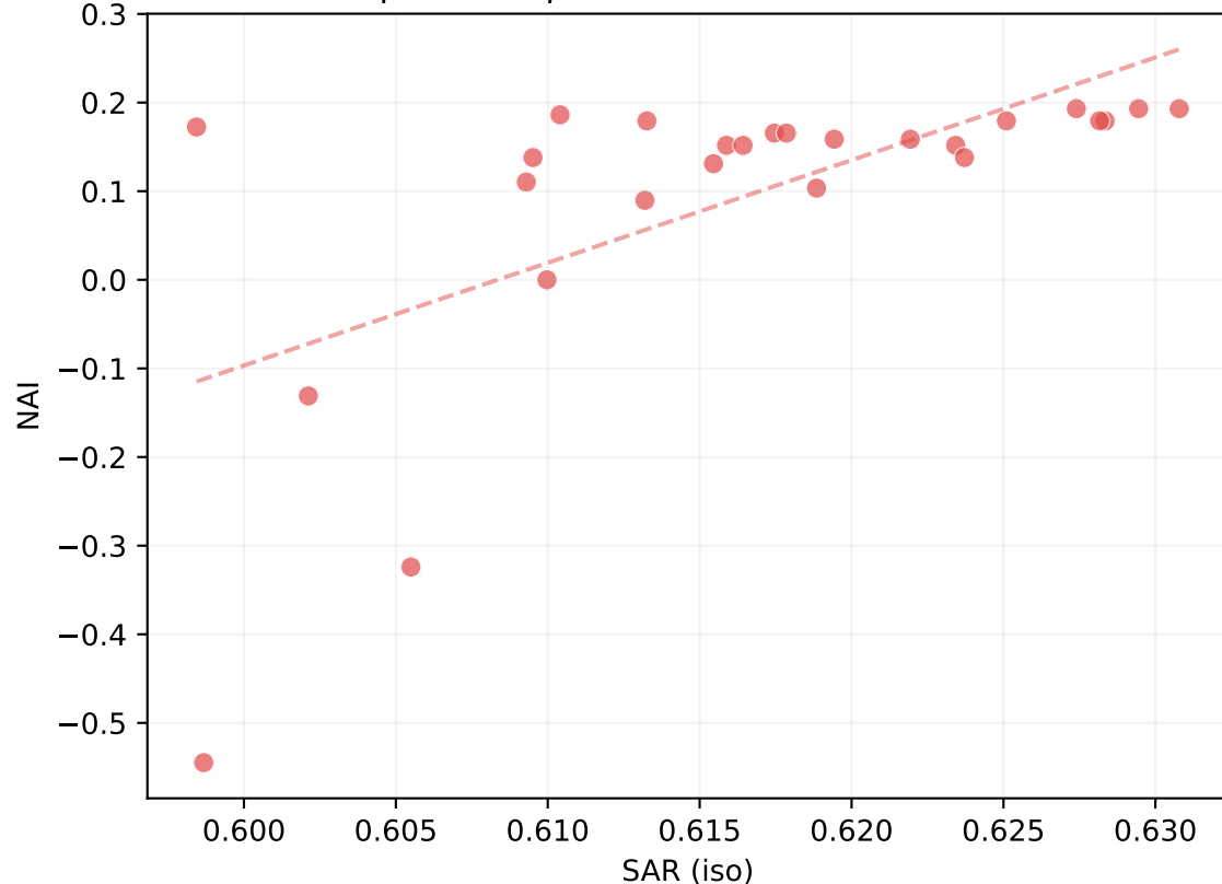
cola Spearman \rho=0.658 , Pearson r=0.622
