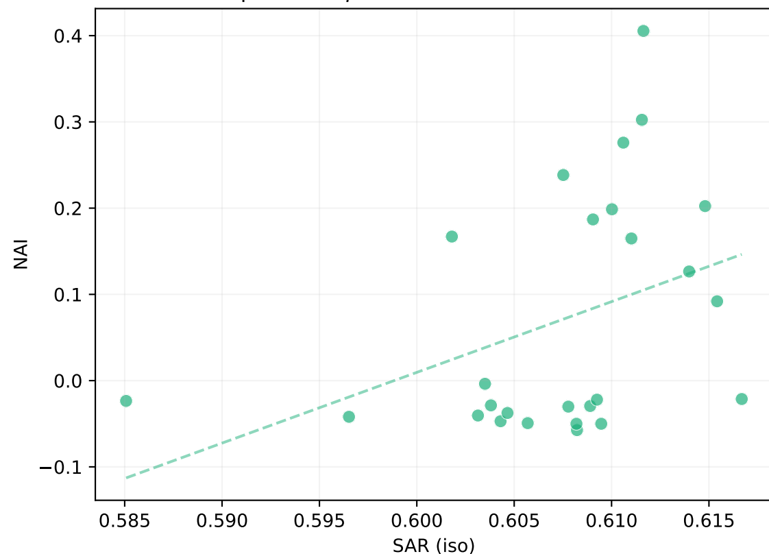
boolq Spearman \rho=0.467 , Pearson r=0.383
