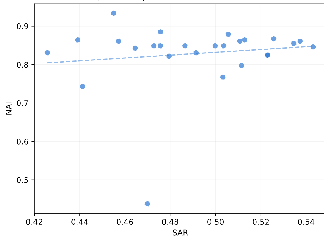
mrpc Spearman \rho=0.072 , Pearson r=0.135
