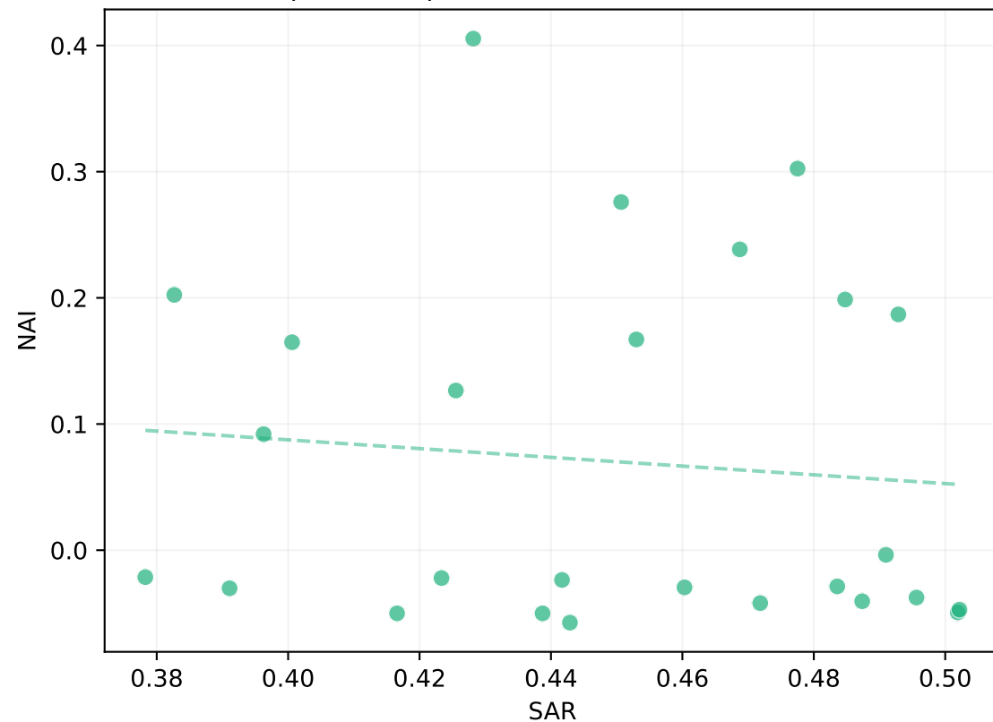
boolq Spearman \rho=-0.149 , Pearson r=-0.098
