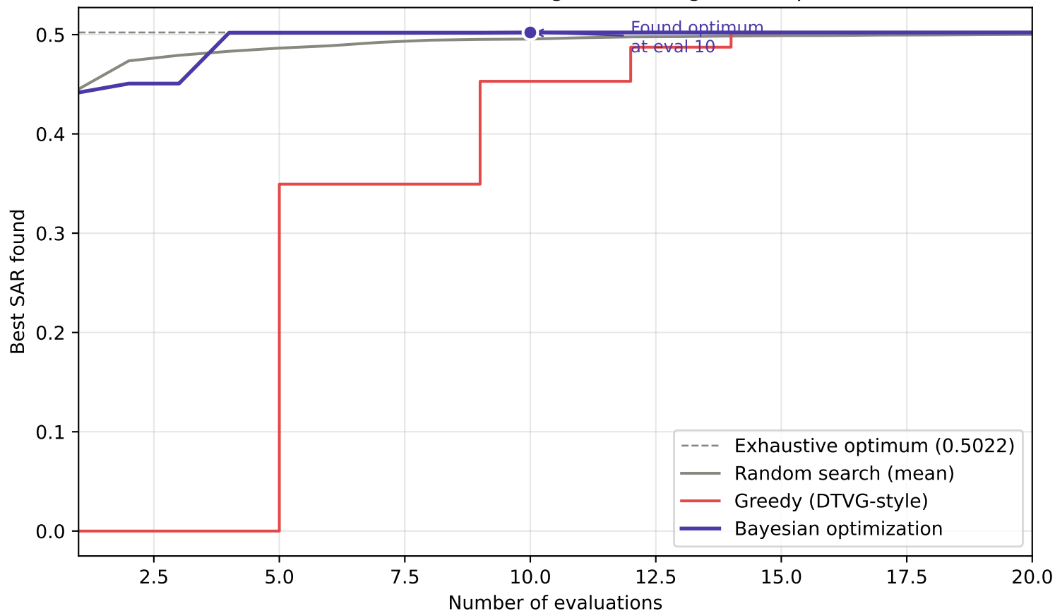
Task selection convergence — target: boolq
