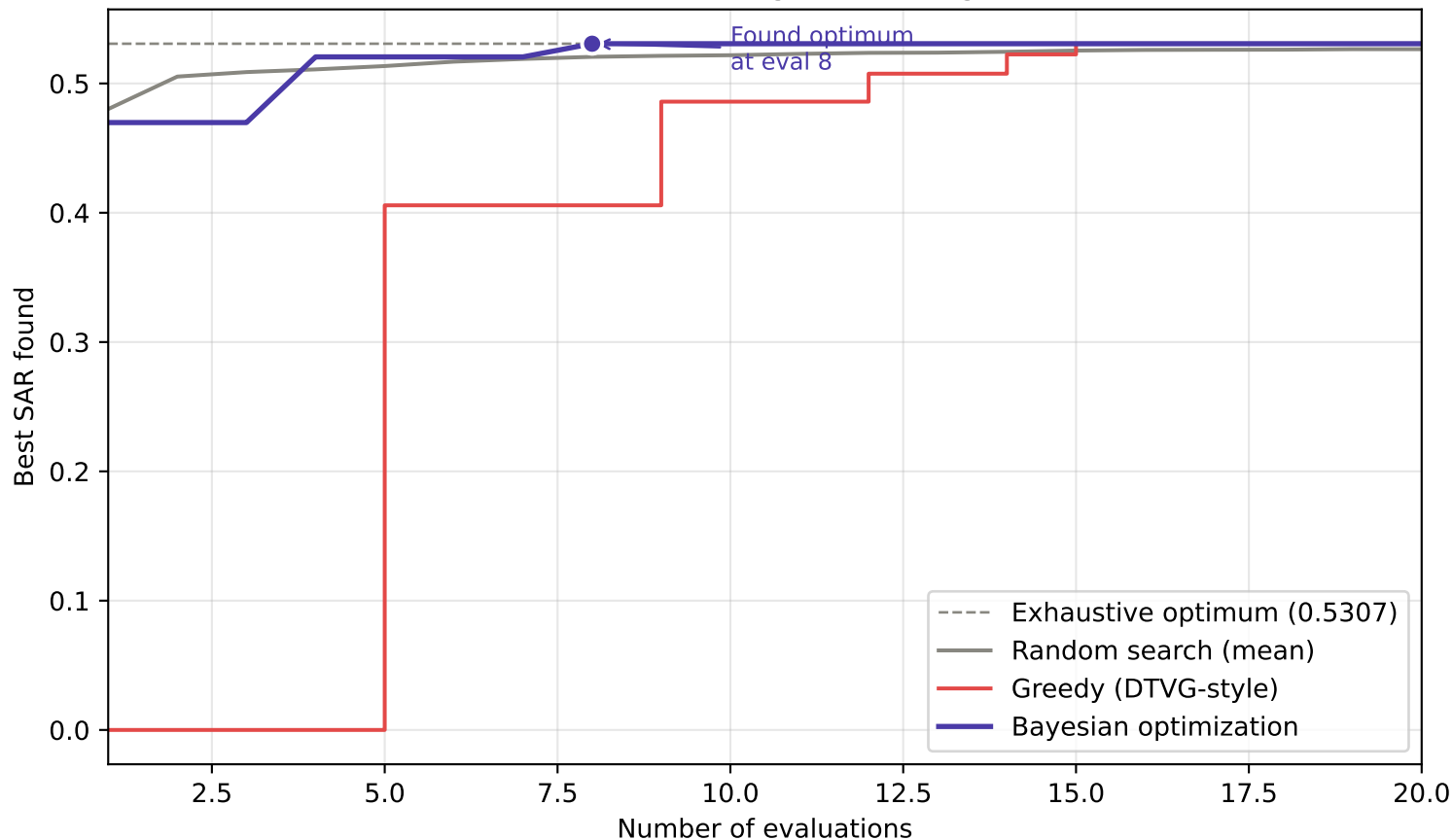
Task selection convergence — target: cola
