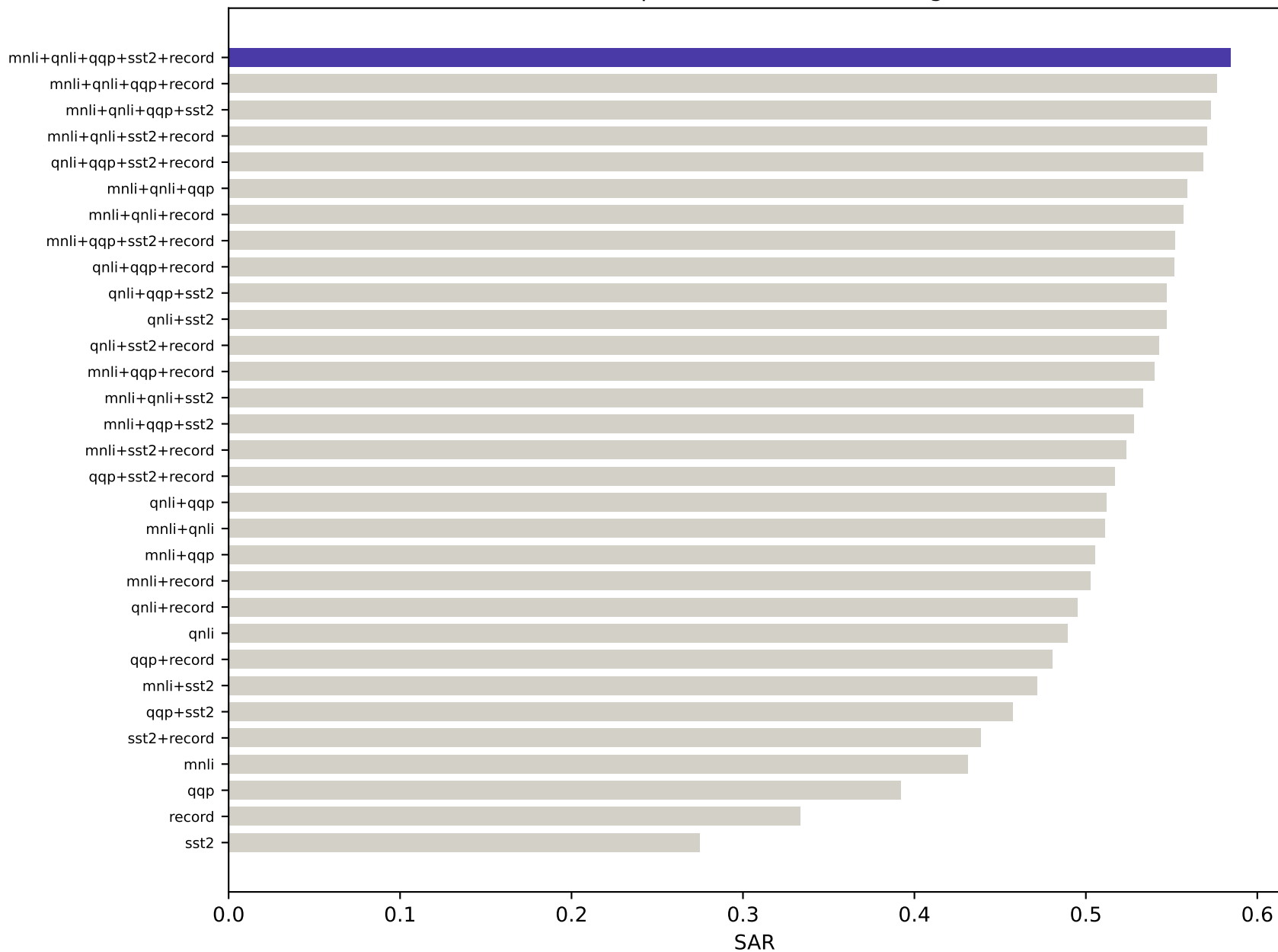
SAR landscape, all 31 subsets — target: rte
