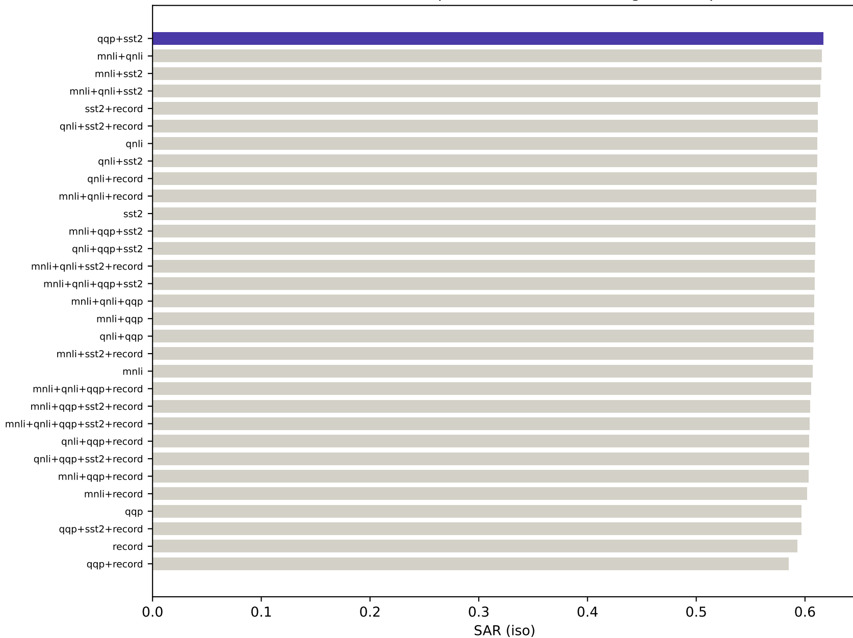
SAR (iso) landscape, all 31 subsets — target: boolq
