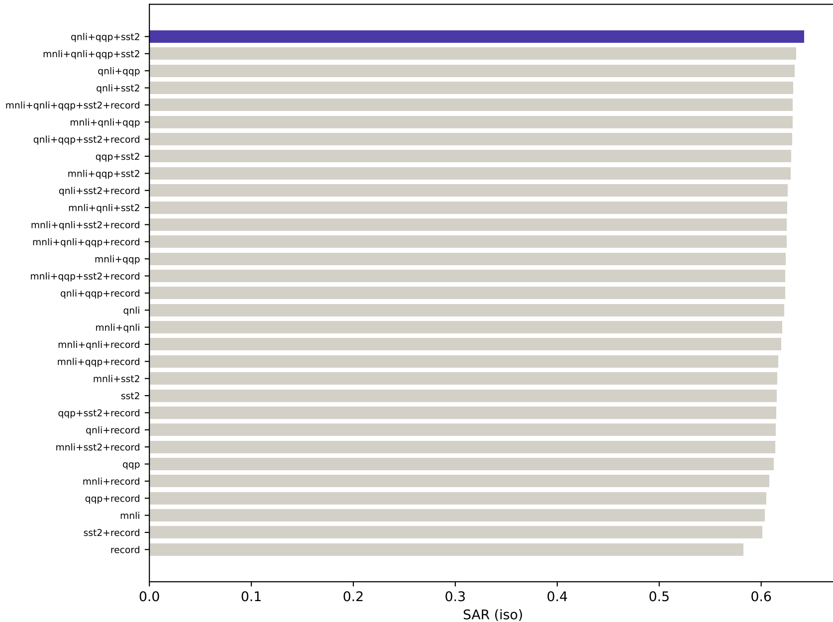
SAR (iso) landscape, all 31 subsets — target: mrpc
