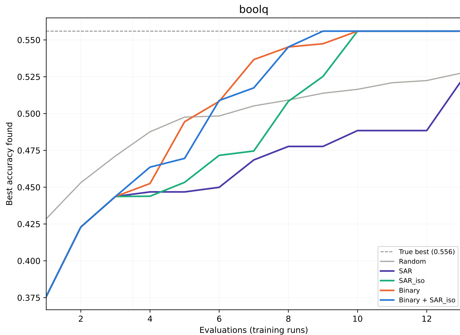
BO convergence by GP feature set
