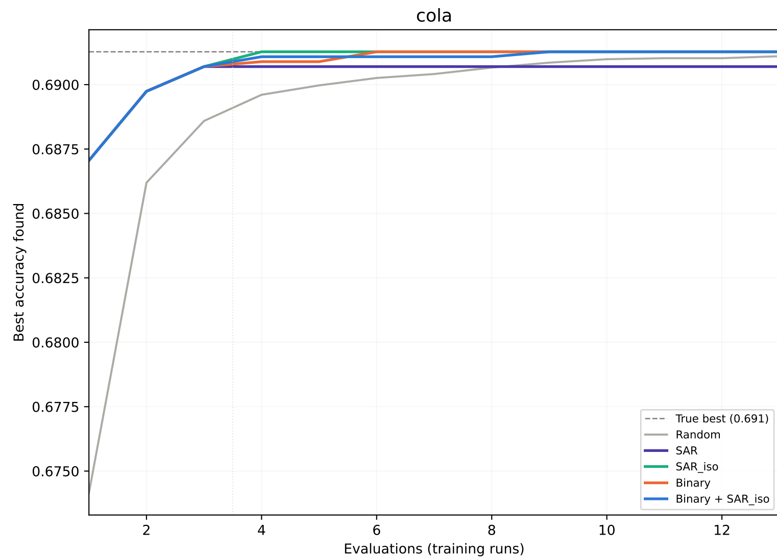
BO convergence by GP feature set
