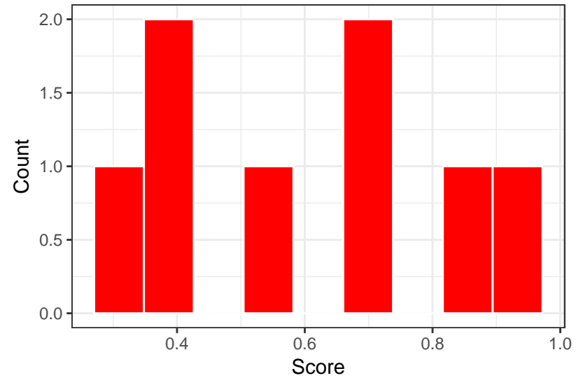
Inefficient DMUs distribution
