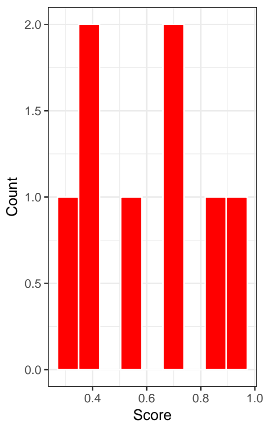
Inefficient DMUs distribution
