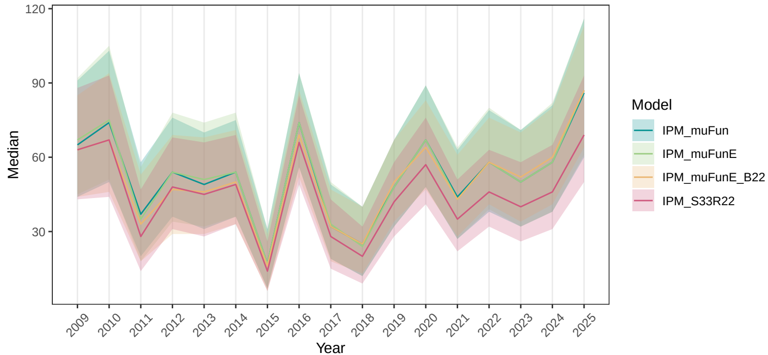
# of young-at-foot
