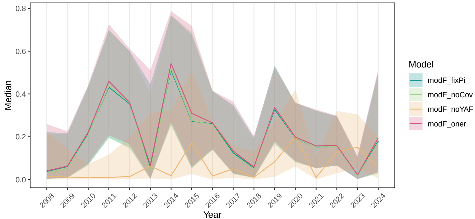
Movement probability (YAF)
