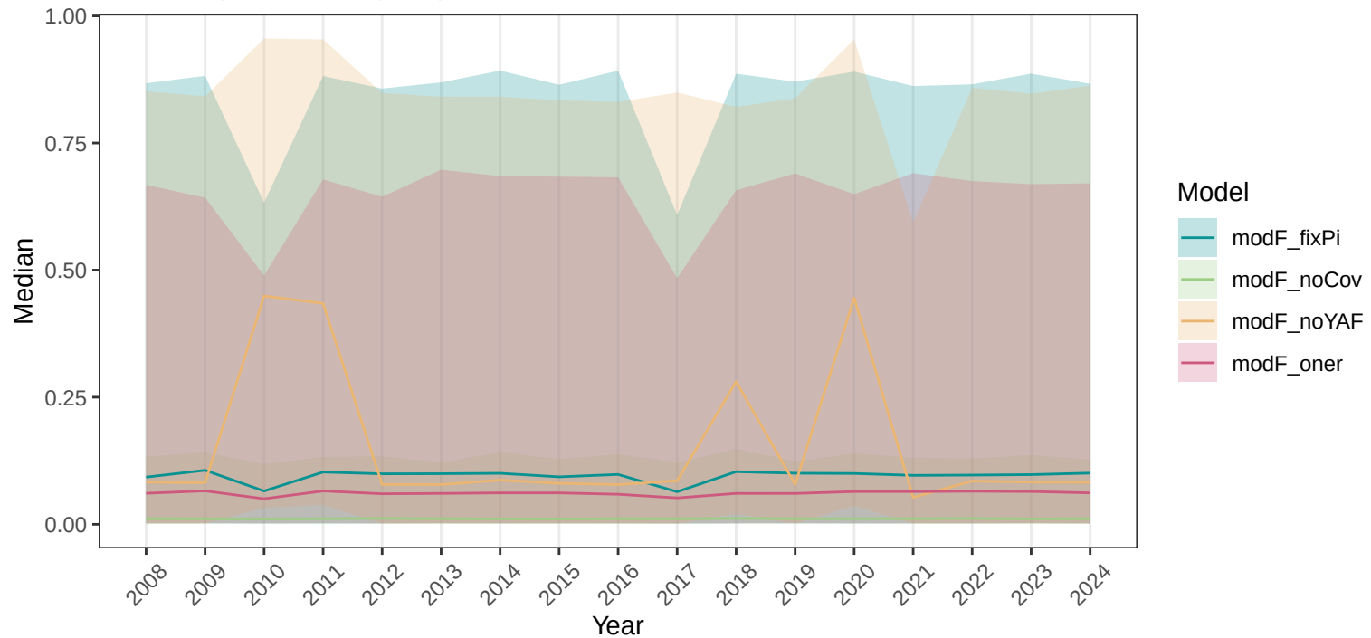
Roadkill probability (YAF)
