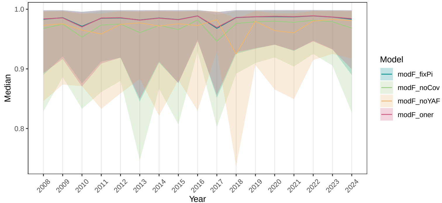
Survival probability (YAF)
