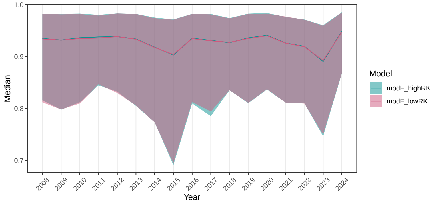
Survival probability (2)
