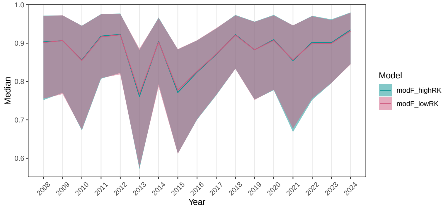
Survival probability (7–9)
