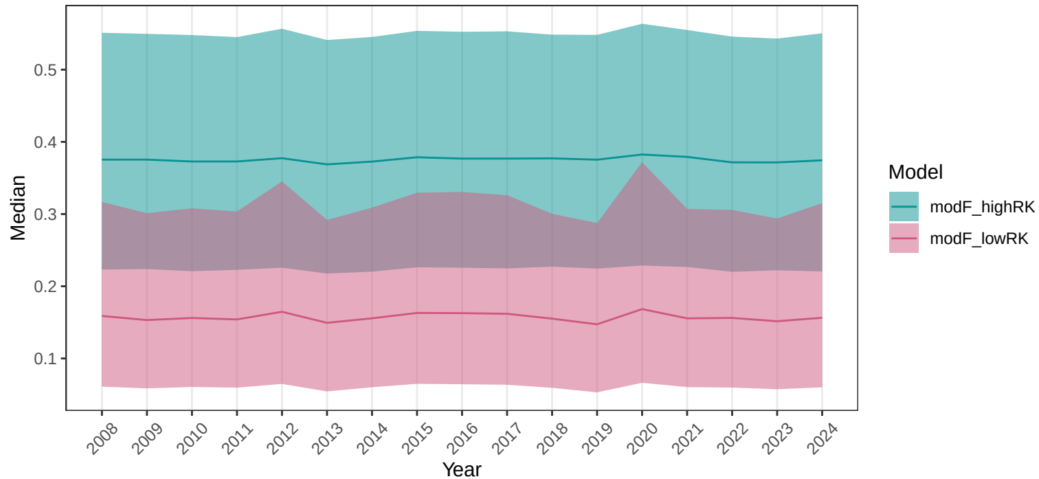
Roadkill probability (1)
