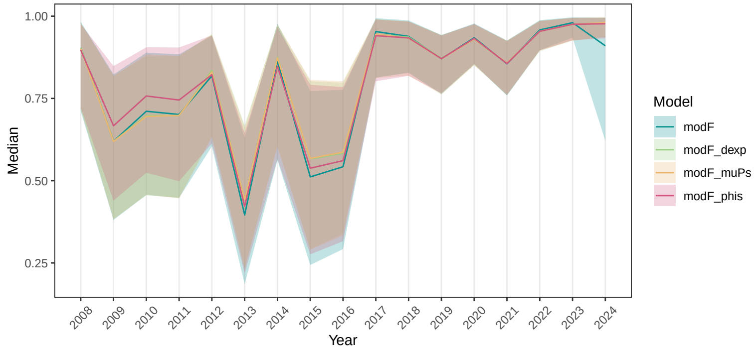
Survival probability (10+)
