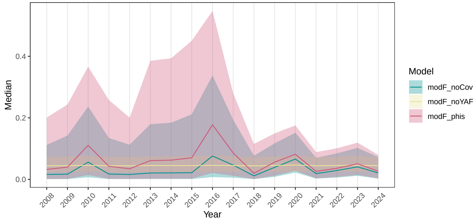
Movement probability (10+)
