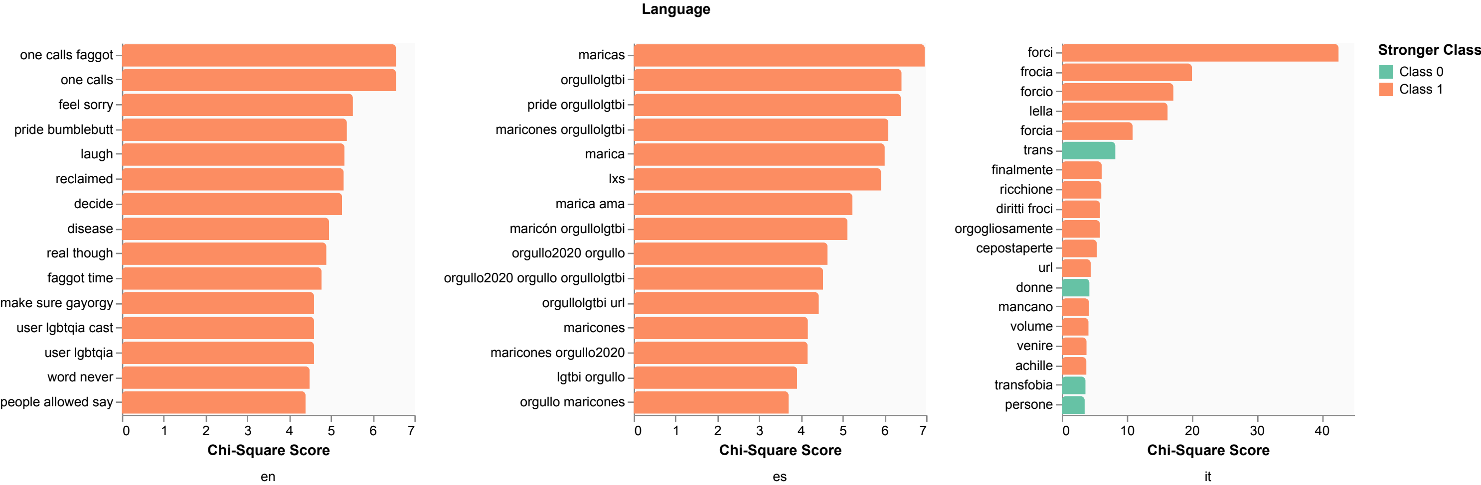
Top Discriminative N-grams per Language (Chi-Square Feature Selection)
