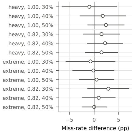
a H1: Diffusion-RB minus GAN-RB
