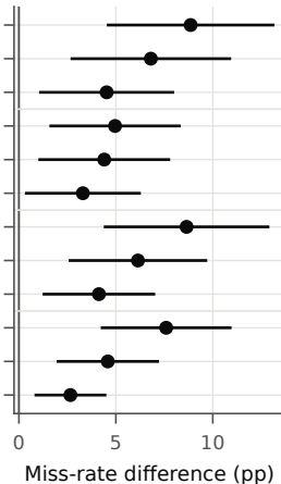
b H2: Diffusion-RB minus QuantileMLP-RB
