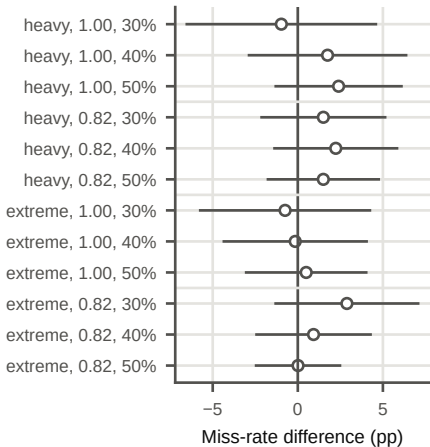
a H1: Diffusion-RB minus GAN-RB
