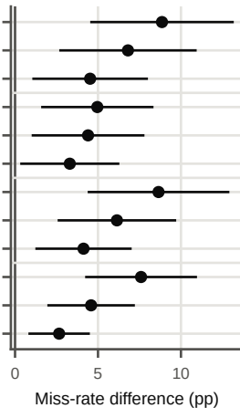
b H2: Diffusion-RB minus QuantileMLP-RB
