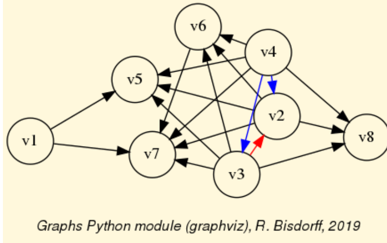
Fig. 6.17: Transitive neighbourhoods of the dual graph -g
