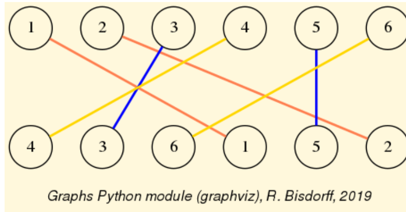
Fig. 6.13: Colored matching diagram of the permutation [4, 3, 6, 1, 5, 2]
