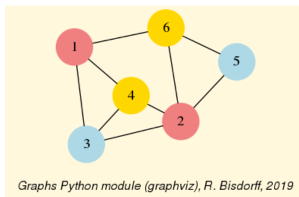
Fig. 6.12: Minimal vertex coloring of the permutation graph
