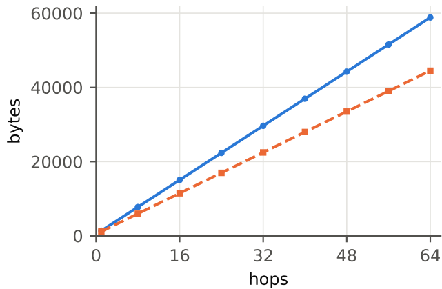
Deposit d_n
