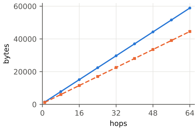
Payment p_i
