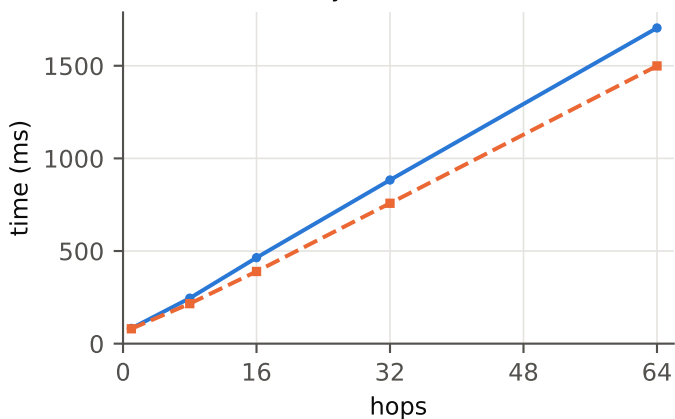
Payee (server)
