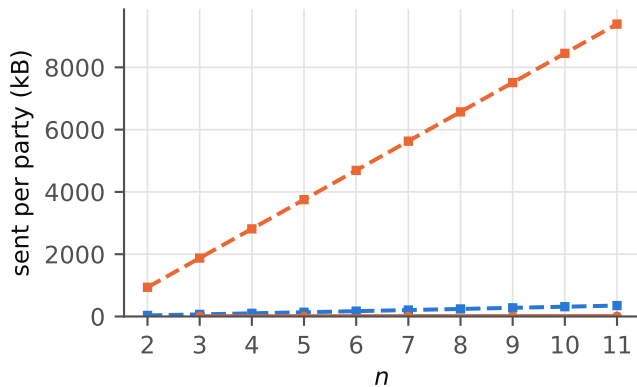
KeyGen
