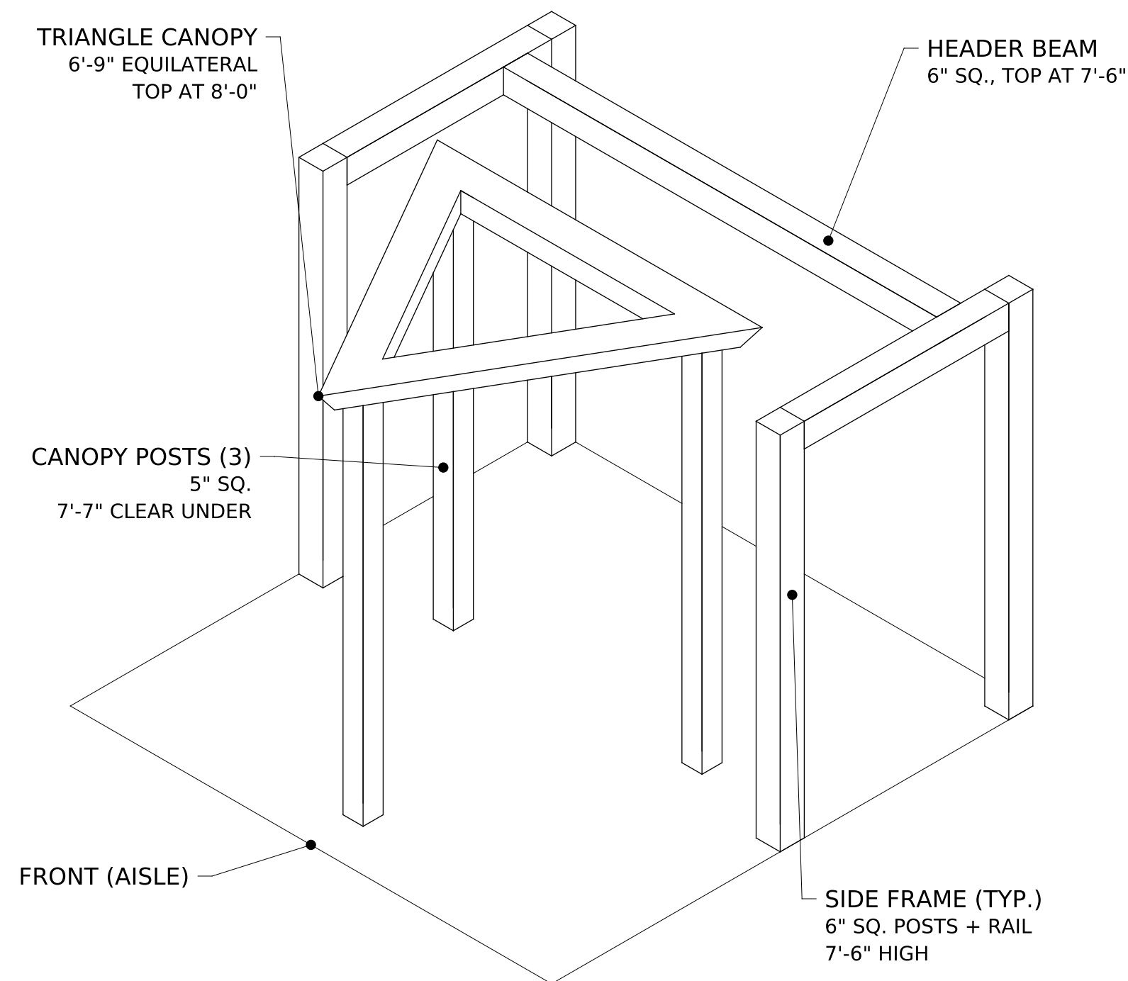
ISOMETRIC VIEW NOT TO SCALE
