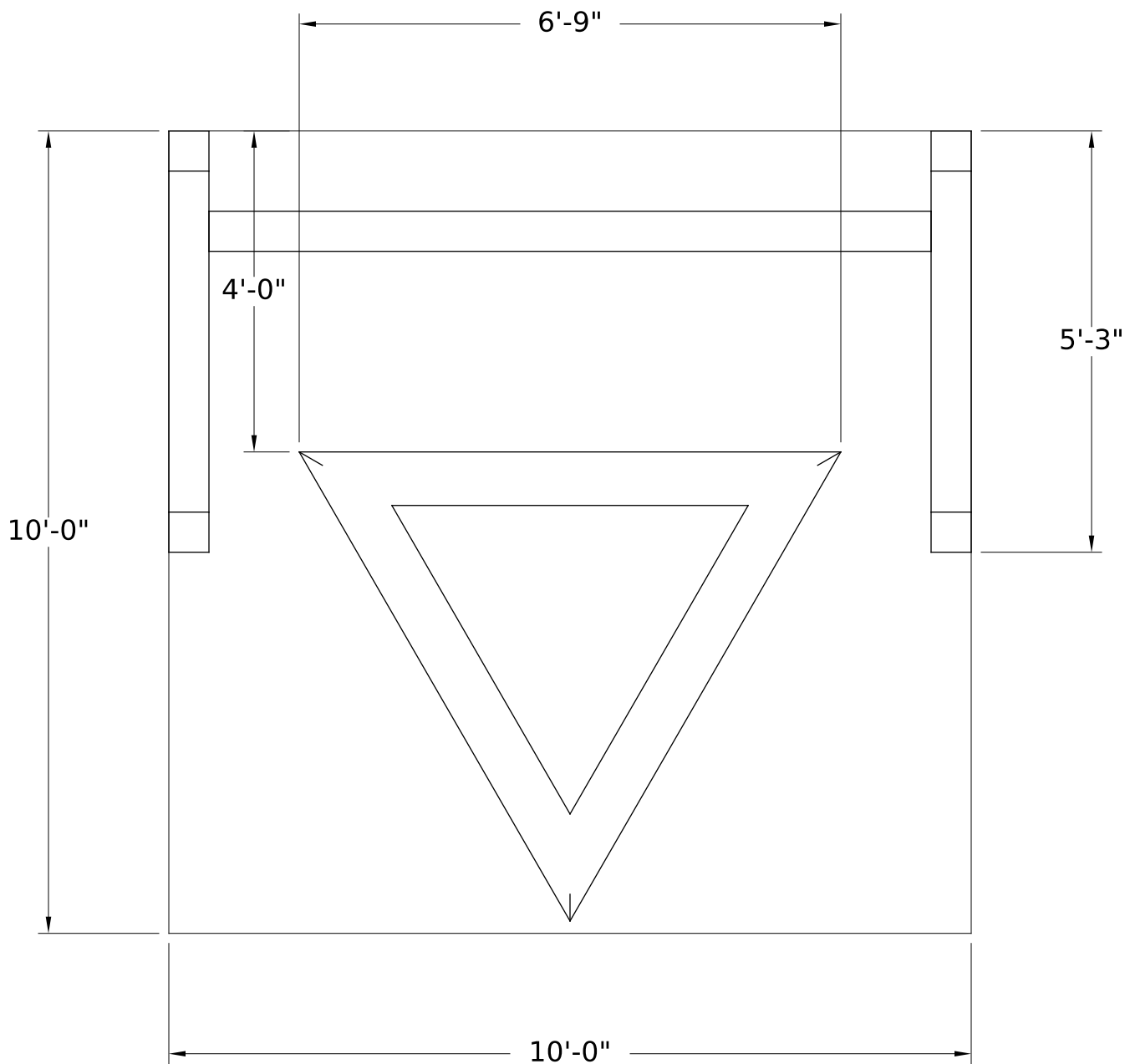
AISLE PLAN VIEW SCALE: 1/2" = 1'-0"
