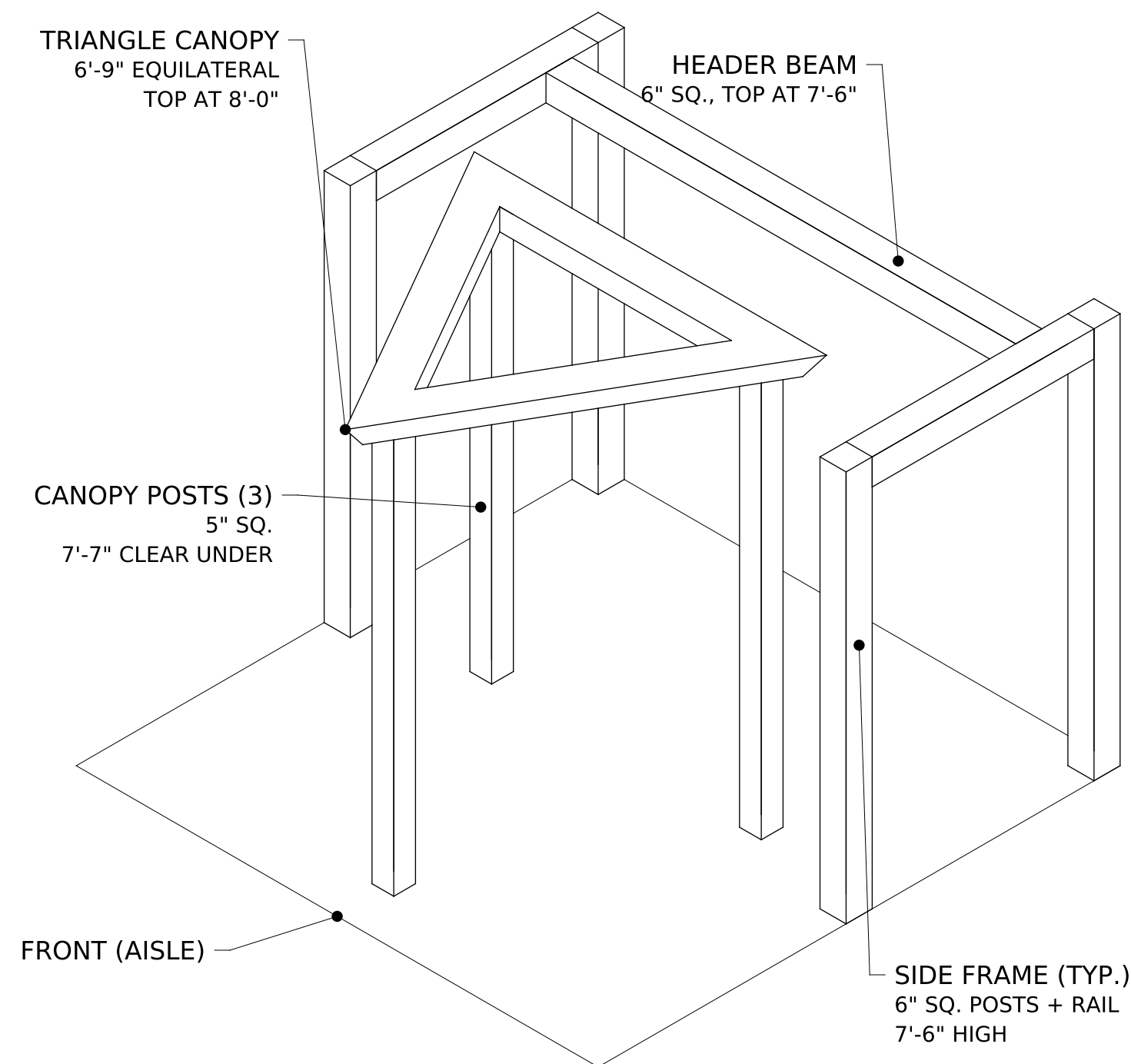
ISOMETRIC VIEW NOT TO SCALE
