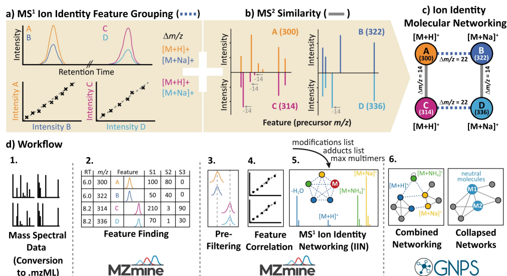
Figure 7: This example of Global Natural Product Social (GNPS) molecular networking illustrates the relationships between different molecular features but this is not fitted for environmental samples which causes gaps. 16
