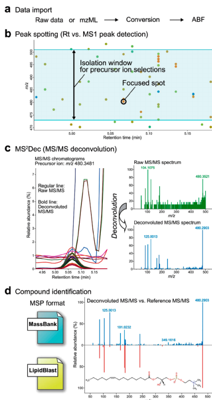
Figure 4: This workflow illustrates data independent acquisition (DIA) using MS Dial while different from our data dependent acquisition (DDA) we are seeking something similar. 21
