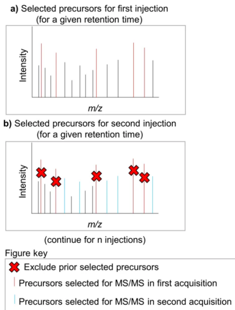
Figure 3: Example of exclusion and inclusion of features to establish our lists. 20
