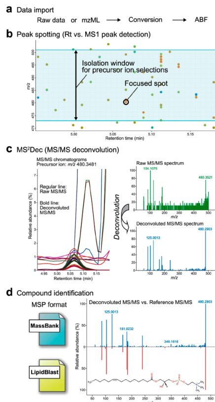
Figure 4: This workflow illustrates data independent acquisition (DIA) using MS Dial while different from our data dependent acquisition (DDA) we are seeking something similar. 18
