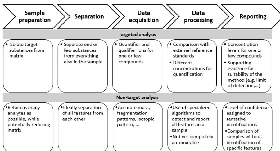
Figure 1: Comparison of non-targeted analysis (NTA) and targeted analysis (TA) approaches for identification of organic contaminants. 24
