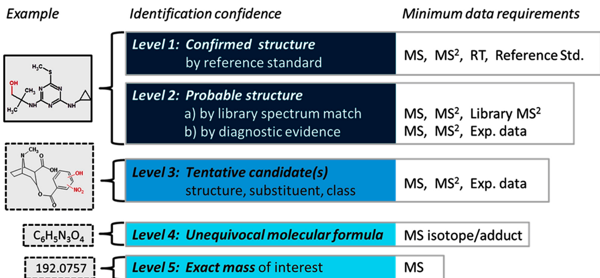
Figure 5: Confidence levels example for molecular feature identification based on the Schymanski framework. 3
