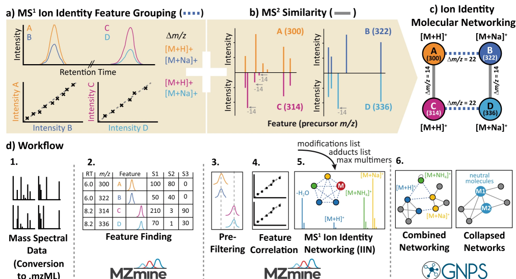
Figure 9: This figure illustrates the GNPS molecular networking approach. It first connects and sorts ions, then annotates them based on their spectral similarities and finally proposes a structure. 16
