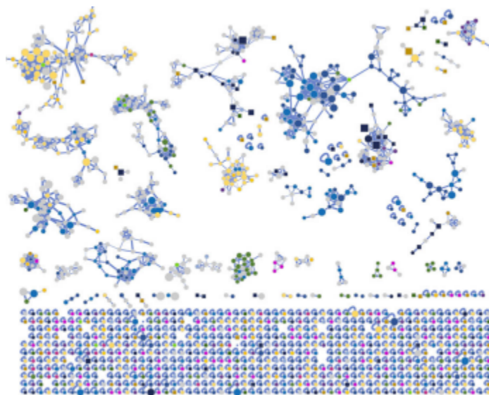
Figure 12: This feature based graph shows how ions become connected in a molecular network based on their similarity, facilitating the identification of unknown compounds. 16 The colors in the graph are by ion identities.
