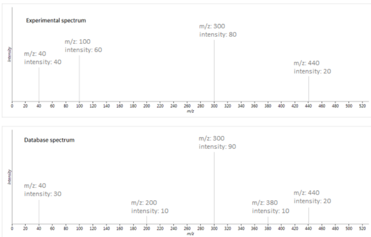
Figure 10: This example illustrates how the experimental spectrum (E) and database spectrum (D) are compared using cosine similarity scoring based on their fragment ion m/z values and intensities. 17,28
