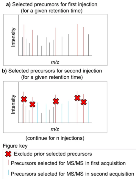
Figure 5: Example of exclusion and inclusion of features to establish our lists. 20
