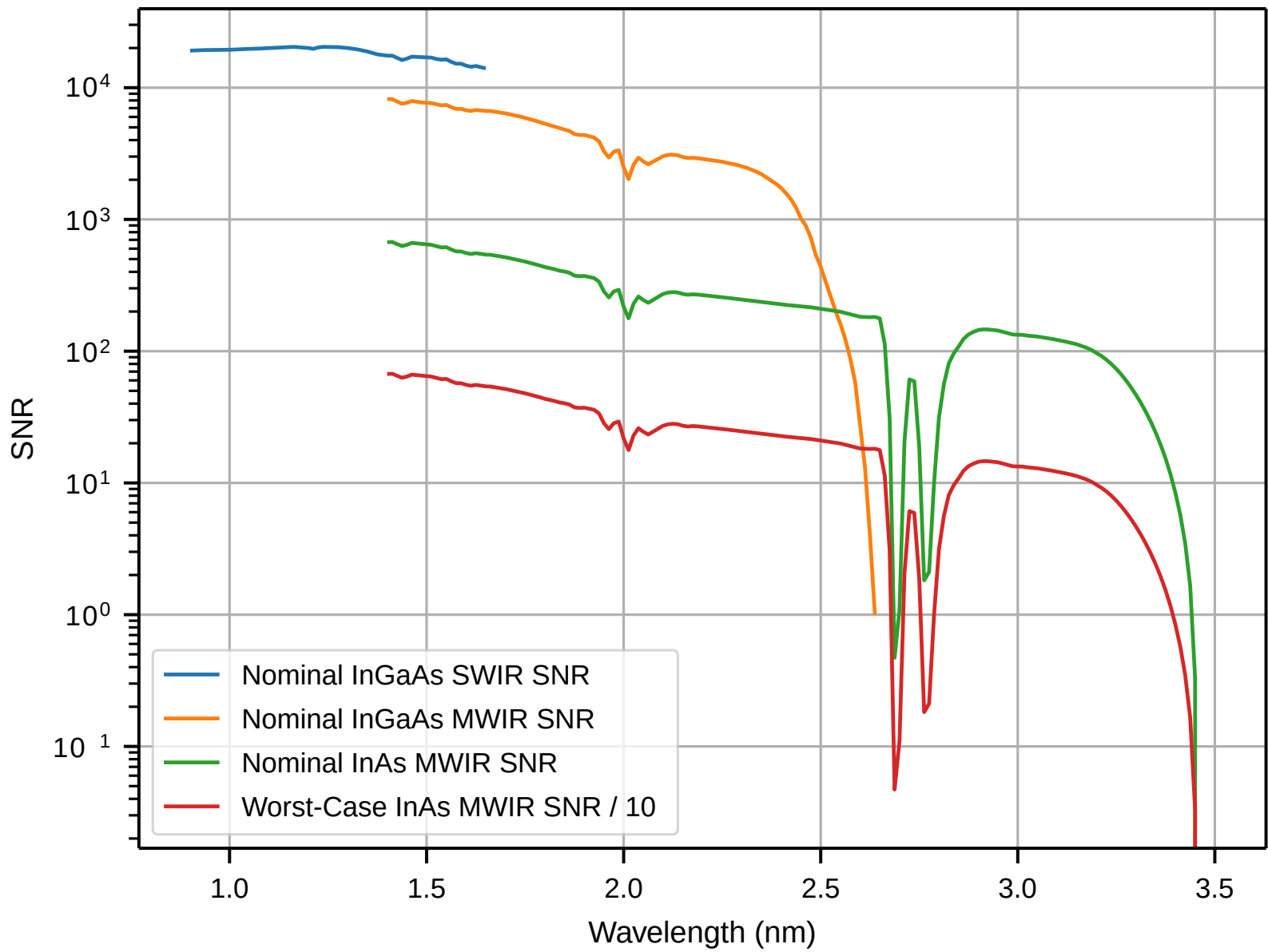
Spectral SNR of InGaAs SWIR and InGaAs & InAs MWIR Sensors
