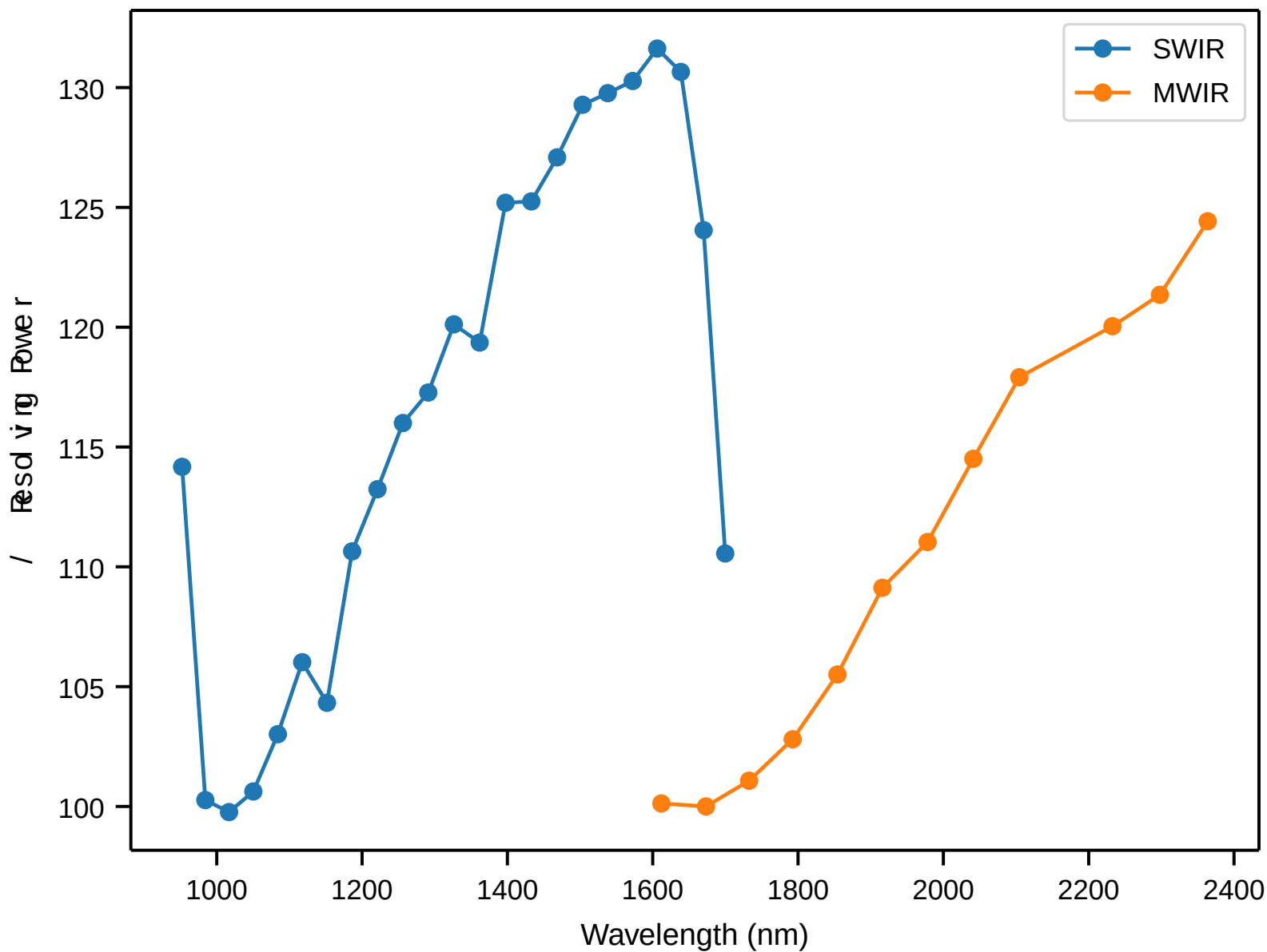
Enfys SWIR & MWIR Spectral Resolving Power [ ]
