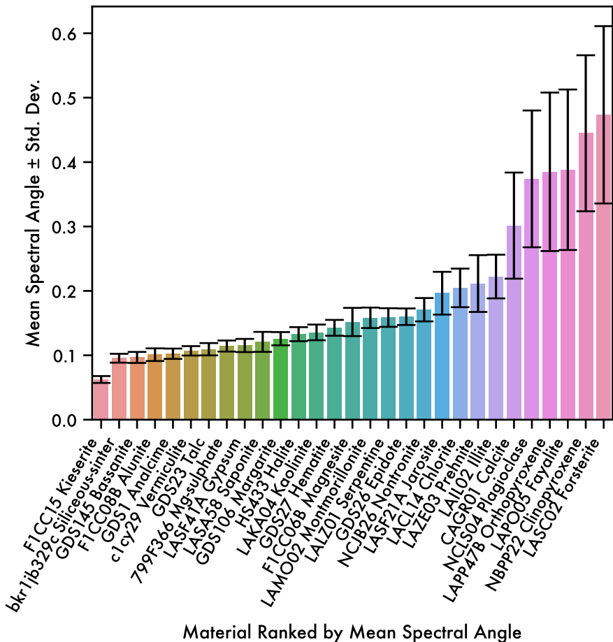
Mean Spectral Angle of N-repeat Noisy Samples vs Clean Spectra Enfy's InAs MWIR
