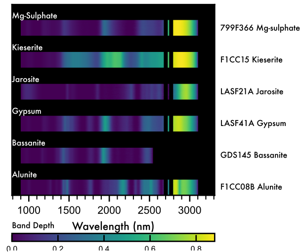
Q. Hydrous_Sulphates
