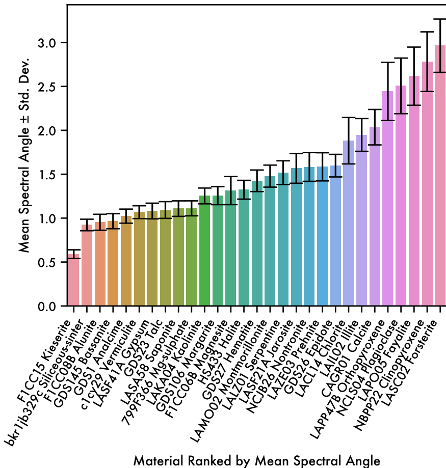
Mean Spectral Angle of N-repeat Noisy Samples vs Clean Spectra Enfys InAs MWIR SNR/10
