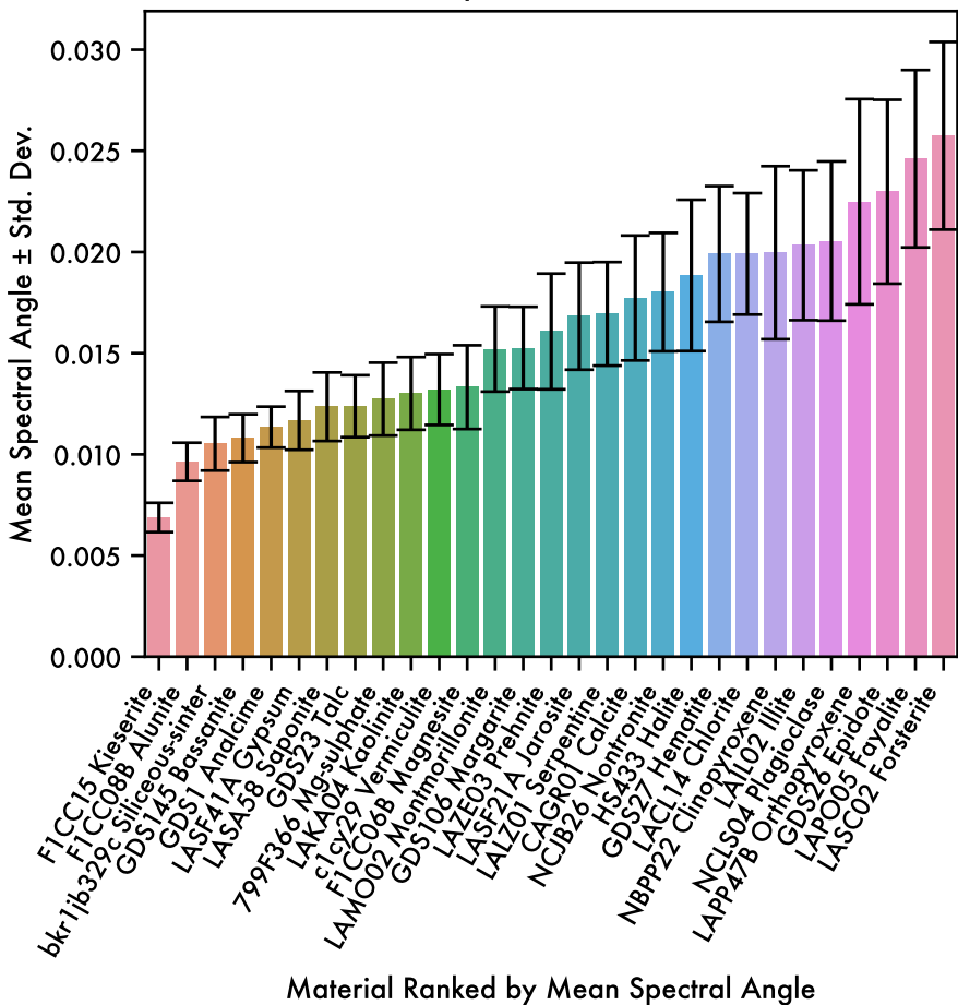
Mean Spectral Angle of N-repeat Noisy Samples vs Clean Spectra Enfys InGaAs MWIR
