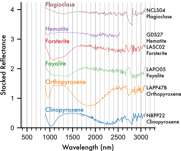
C. Iron Oxides & Primary Silicates
