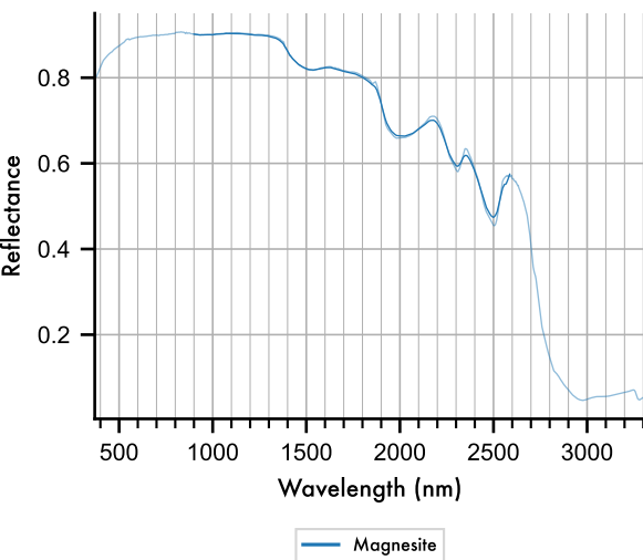
C. Hs433
