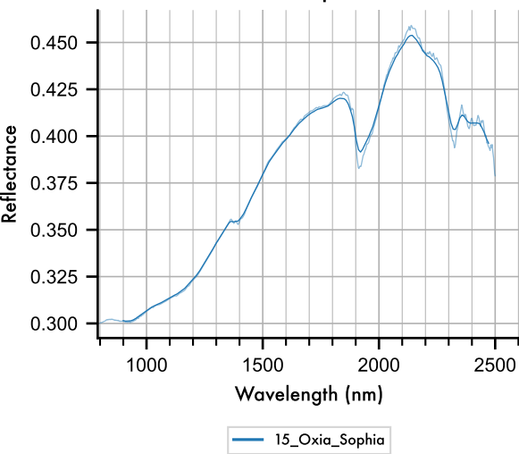
I. 15_Oxia_Sophia_00001
