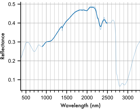
Chlorite
