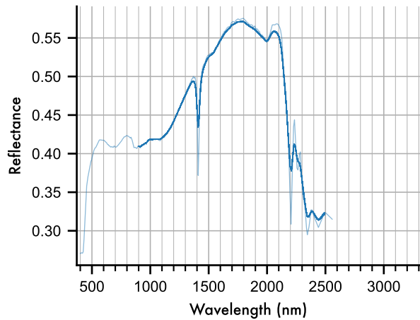
Margarite
