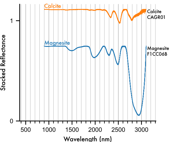
C. Carbonates
