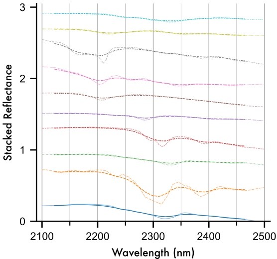
C. Phyllosilicates
