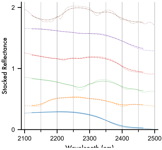
C. Phyllosilicates
