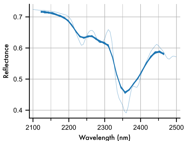
Prehnite
