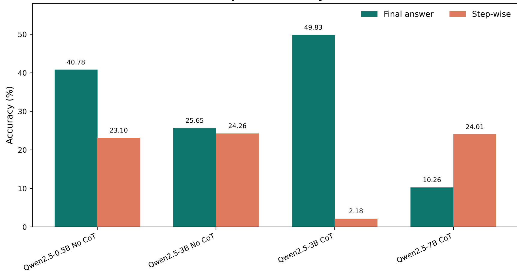
Final-answer versus canonical step-wise accuracy
