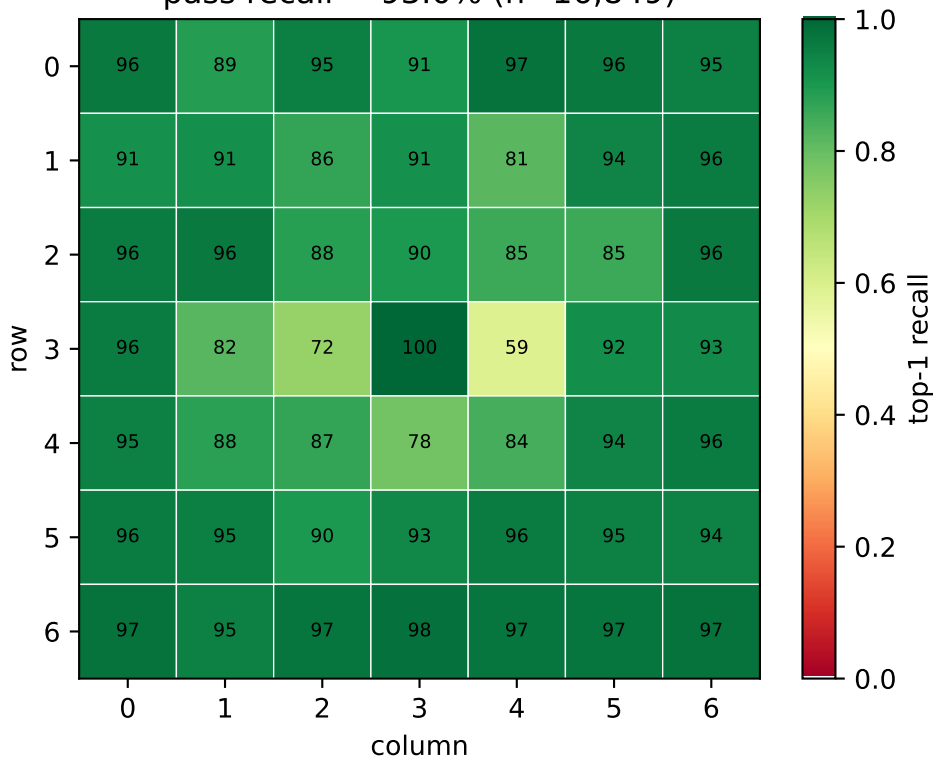
Champion per-point top-1 recall (val) pass recall = 93.0% (n=16,849)
