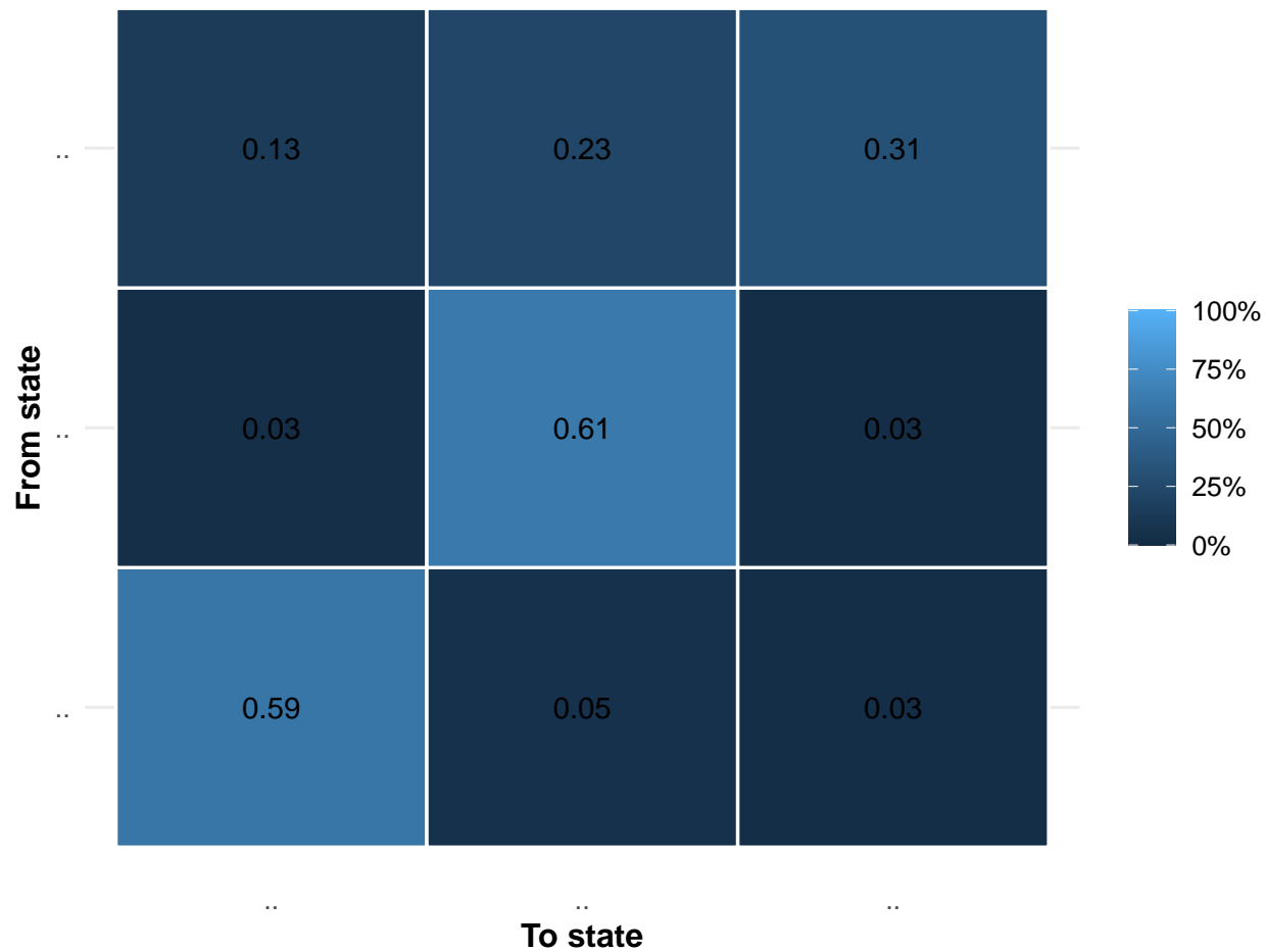
Transition probabilities (average) (K = 3, mod=1)
