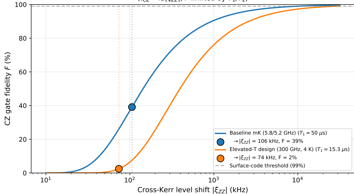
CZ free-evolution fidelity vs |\xi_{ZZ}| ( t_{CZ} = \pi/|\xi_{ZZ}| , F limited by T_1/T_2 )
