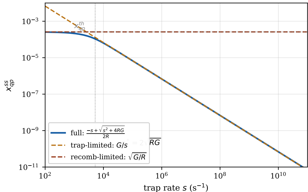
(b) steady state across crossover
