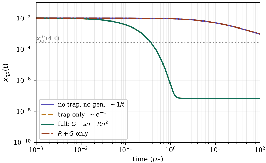
(a) dynamic decay regimes
