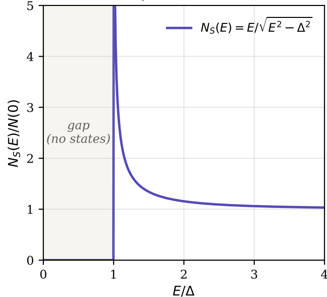
(b) BCS density of states
