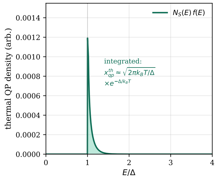
(c) population = N_S \times f
