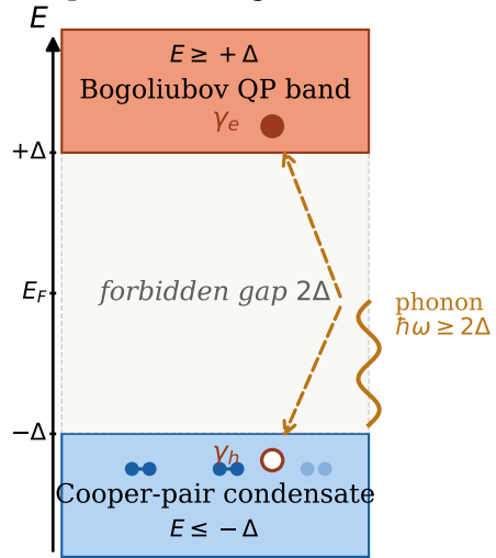
(a) pair breaking
