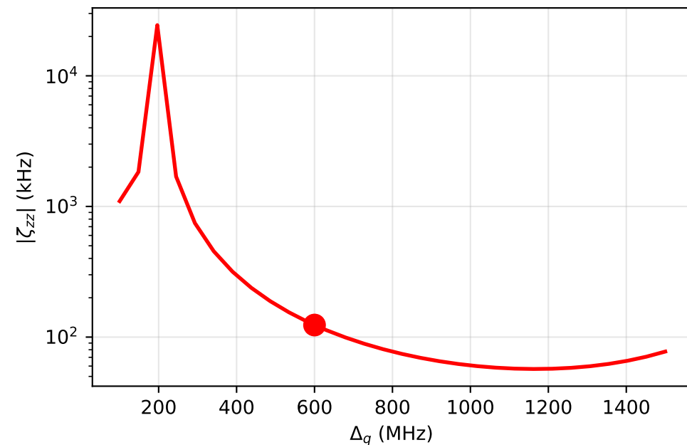
B. Static parasitic cross-Kerr (smaller is better)
