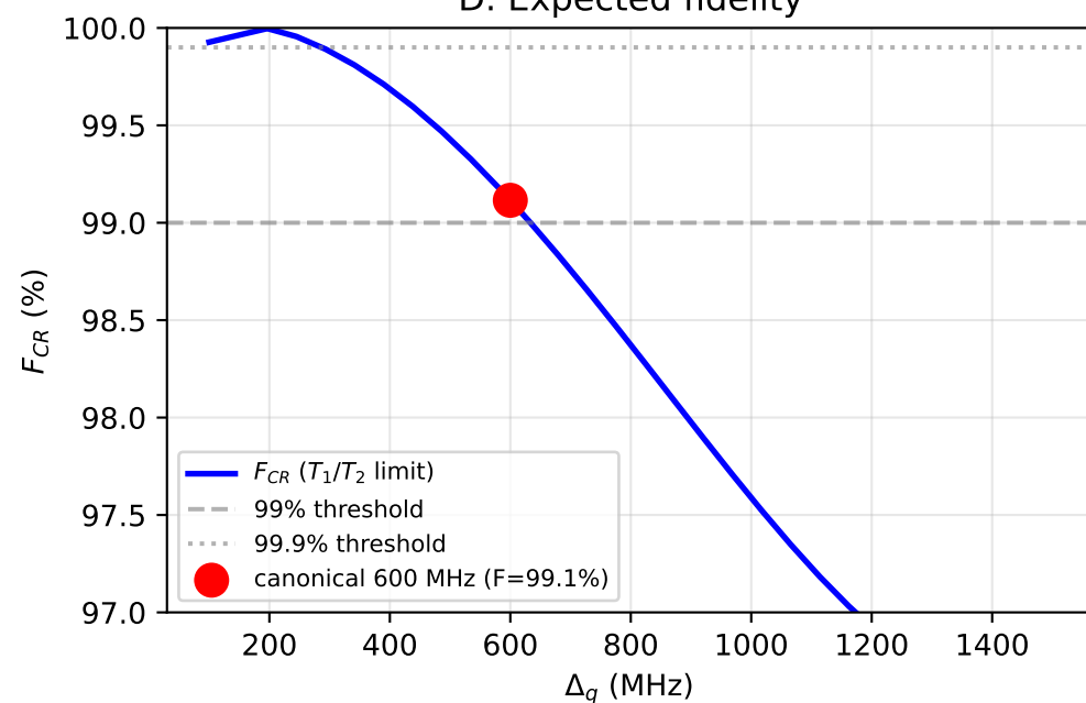
D. Expected fidelity
