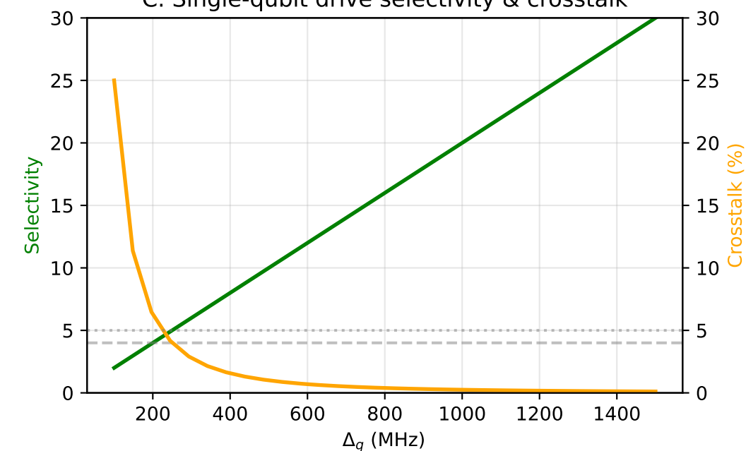
C. Single-qubit drive selectivity & crosstalk
