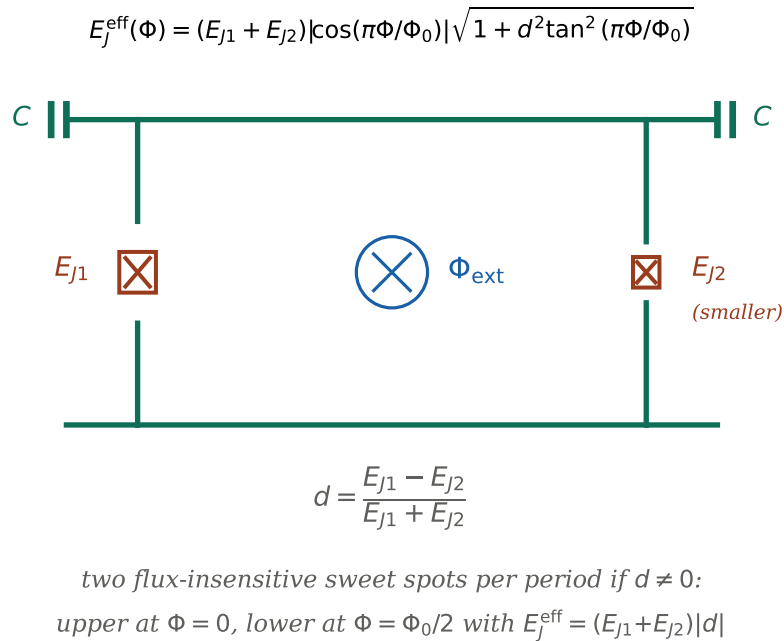
(b) asymmetric SQUID with external flux \Phi_{\text{ext}}
