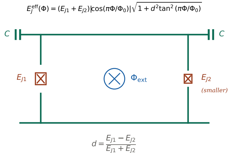
(b) asymmetric SQUID with external flux \Phi_{\text{ext}}
