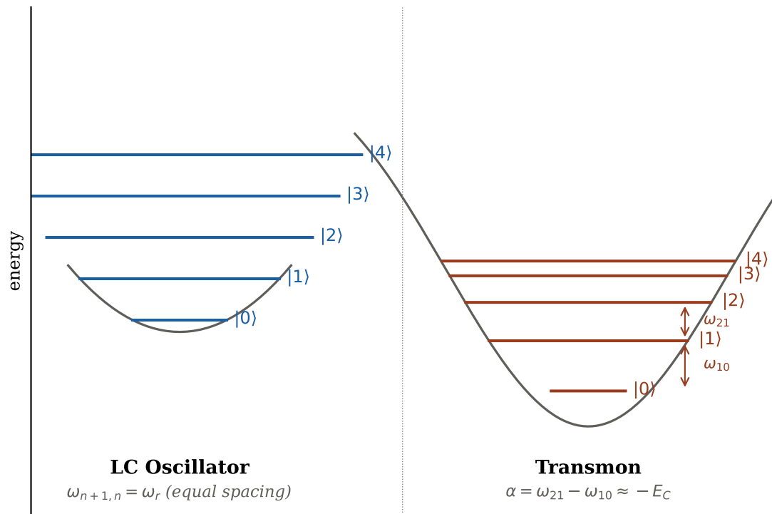
(a) anharmonicity makes the transmon a qubit
